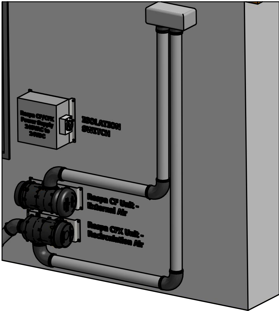
FRONT ISOMETRIC VIEW OF RESPA ASSEMBLY
