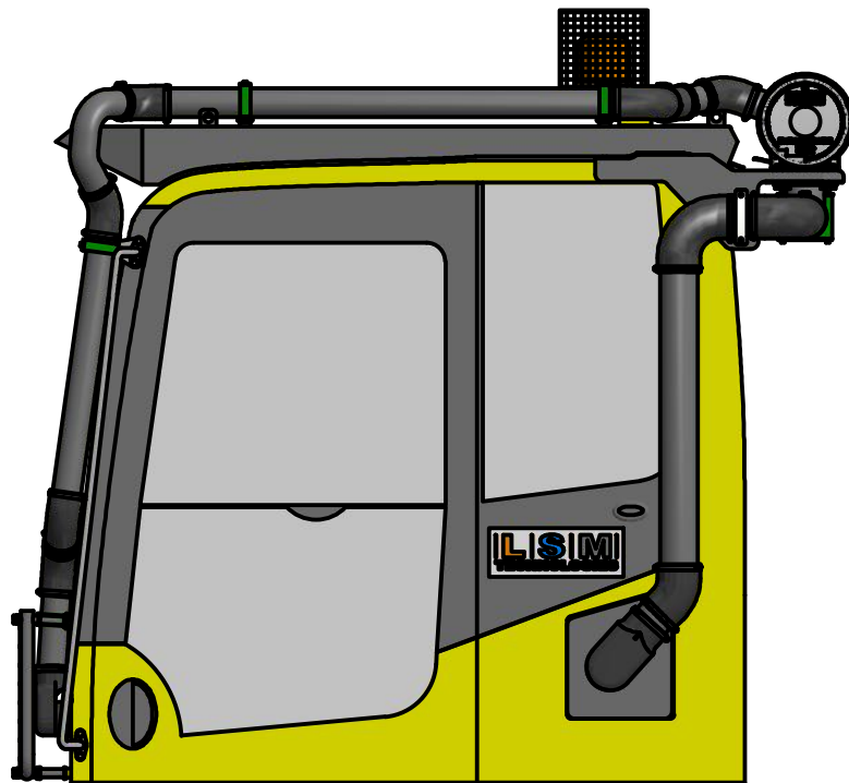
RIGHTHAND SIDE VIEW
