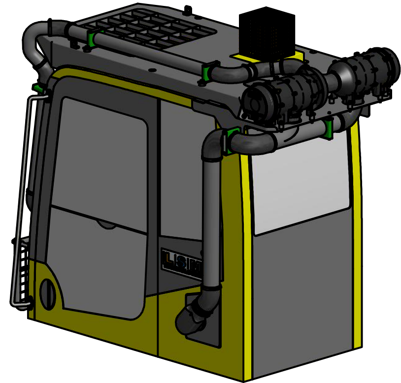
REAR ISOMETRIC VIEW
